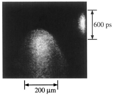
FIG. 1. Rear side shock breakthrough for a 18 \mu\text{m} Al target. Optical smoothing is realized with RPP's giving a measured focal spot diameter FWHM= 106 \mu\text{m} . Time fiducial is on the right of the image.
