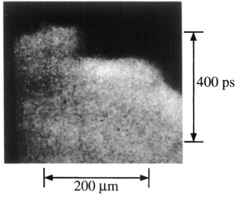
FIG. 4. Rear side shock breakthrough for an Al target with a 7.5 \mu\text{m} basis and a 2.8 \mu\text{m} step. Optical smoothing with PZP's.
