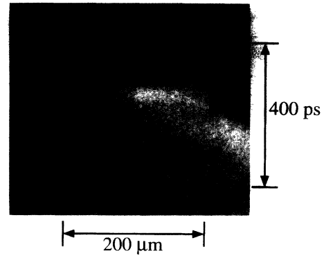
FIG. 4. Rear side shock breakthrough for an Al target with a 7.5 μm basis and a 2.8 μm step. Optical smoothing with PZP’s.
