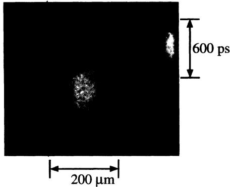
FIG. 1. Rear side shock breakthrough for a 18 \mu\text{m} Al target. Optical smoothing is realized with RPP's giving a measured focal spot diameter FWHM= 106 \mu\text{m} . Time fiducial is on the right of the image.
