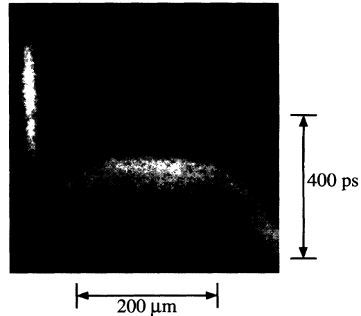
FIG. 2. Rear side shock breakthrough for a 13.8 \mu\text{m} Al target. Optical smoothing is realized with PZP's giving a measured focal spot diameter FWHM= 400 \mu\text{m} . Time fiducial is on the left of the image.
