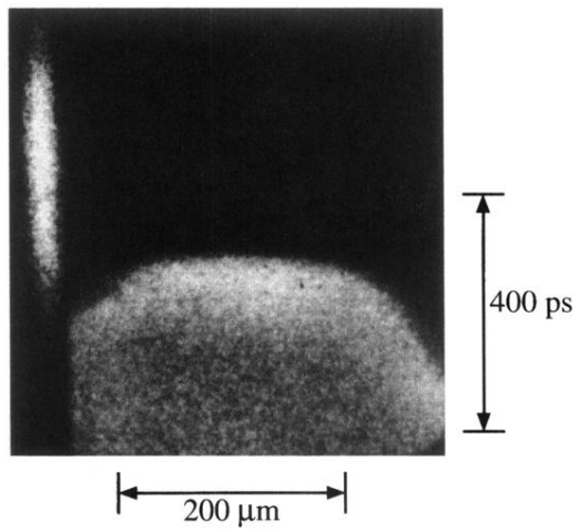
FIG. 2. Rear side shock breakthrough for a 13.8 \mu\text{m} Al target. Optical smoothing is realized with PZP's giving a measured focal spot diameter FWHM= 400 \mu\text{m} . Time fiducial is on the left of the image.
