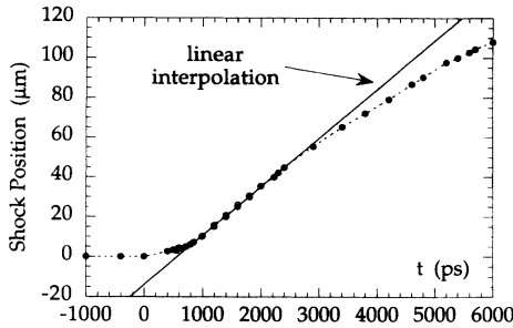
FIG. 3. Shock position as a function of time in Al target according to 1D code FILM simulations ( I_L = 7 \times 10^{13} W/cm 2 , peaked at t = 1 ns, FWHM=600 ps). The linear interpolation corresponds to a shock velocity D = 24 μm/ns.
